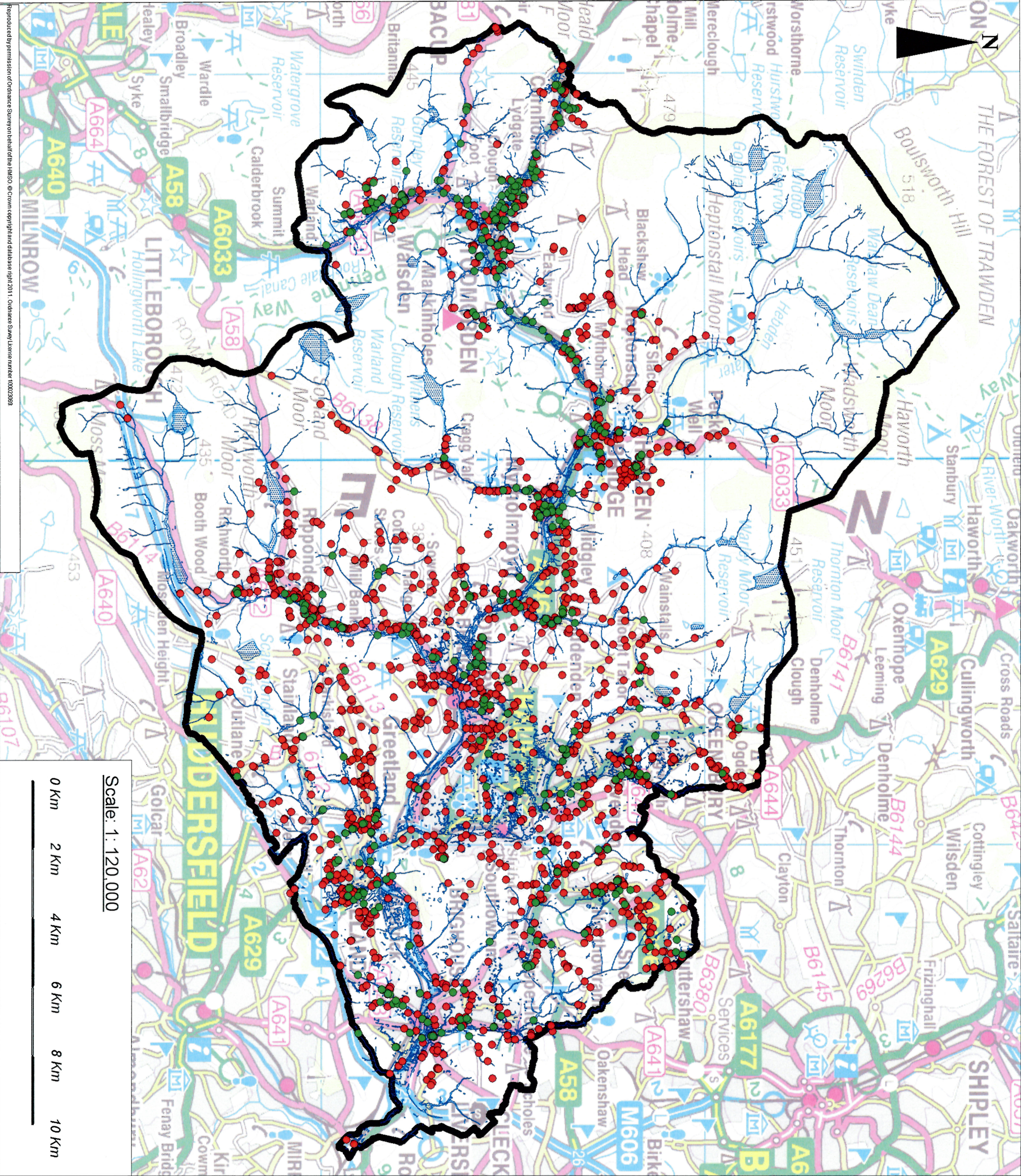
Figure 11 - Surface water flooding locations identified from local knowledge
